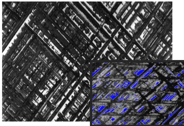
COLORED HIGHLIGHTS REPRESENT PLATE BEARING AREA
